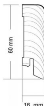
Cubus 60, FR-Profil weiss
