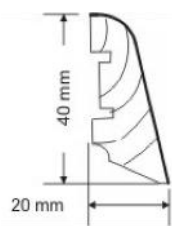
Softline 40, FN-Profil Eiche
